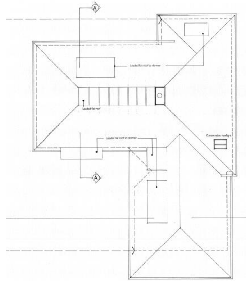
Roof Plan
