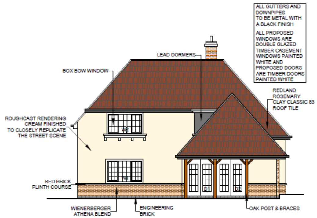
ELEVATION TO SOUTHMEADS ROAD
