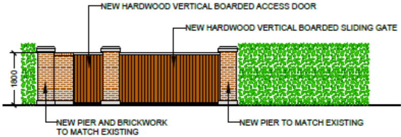
FRONT ENTRANCE DETAIL (SCALE 1:100)
