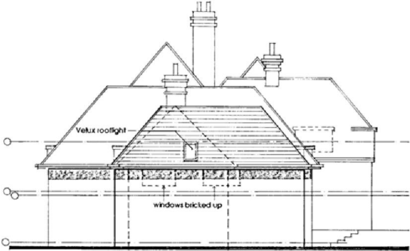
Side elevation to adjacent house
